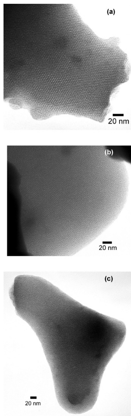
Figure 8. Representative TEM images of (a) C_{16}N(CH_3)(CH_2CH_2OH)_2Pt_4SnTe_4 down the pore tunnel axis, (b) C_{16}N(CH_3)(CH_2CH_2OH)_2Pt_4SnTe_4 perpendicular to the pore tunnel axis, and (c) large particle of C_{16}N(CH_3)(CH_2CH_2OH)_2Pt_4SnTe_4 showing the hexagonal organization extending over its full body.
