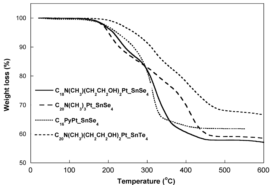
Figure 9. TGA curves of C_{18}N(CH_3)(CH_2CH_2OH)_2Pt\_SnSe_4 , C_{20}N(CH_3)_3Pt\_SnSe_4 , C_{16}PyPt\_SnSe_4 , and C_{20}N(CH_3)(CH_2CH_2OH)_2Pt\_SnTe_4 under nitrogen flow (heating rate 10 deg/min).
