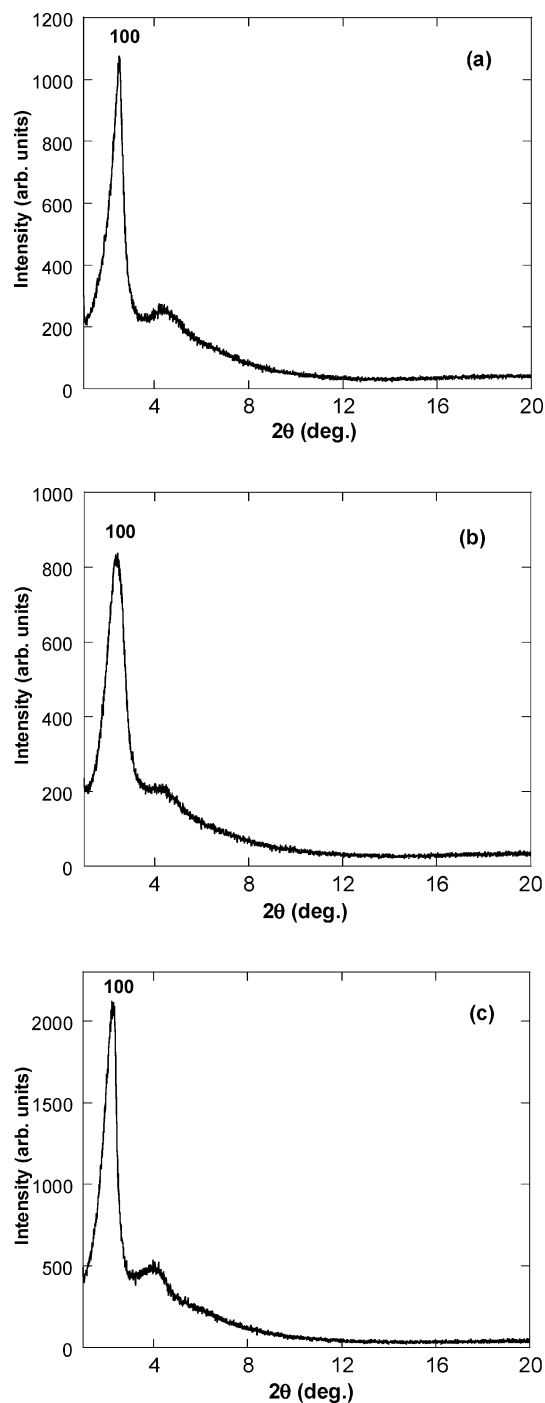
Figure 7. X-ray powder diffraction patterns of C_nN(CH_3)(CH_2CH_2OH)_2Pt_4SnTe_4 (a) n = 16 , (b) n = 18 , and (c) n = 20 .
